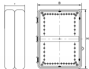
Deckel / cover
