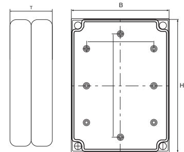
Deckel / Cover
